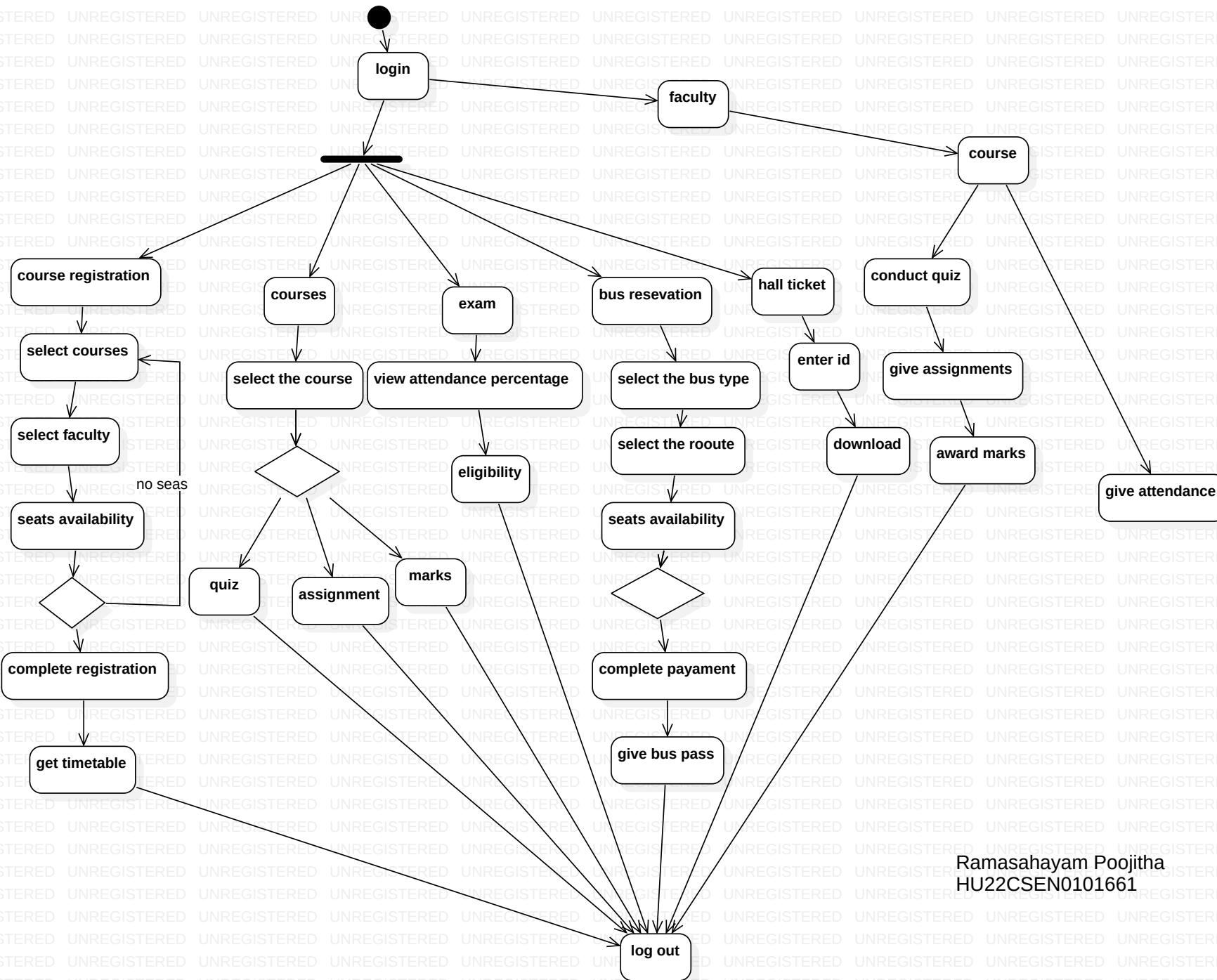
StateMachine1::StatechartDiagram1
